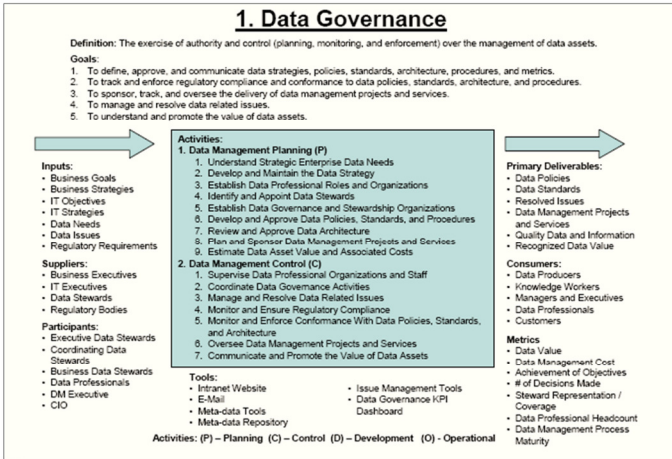
Figure 37: The overview of Data Governance from DMBoK
